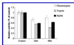
Figure 5. Proteasome activity following exposure to capsaicin. PC3 cells were cultured with capsaicin ( 2 \times 10^{-4} mol/L), harvested at the indicated times and chymotrypsin-like, trypsin-like, and PGPH activities were assayed using appropriate fluorogenic peptides as described in Materials and Methods.
